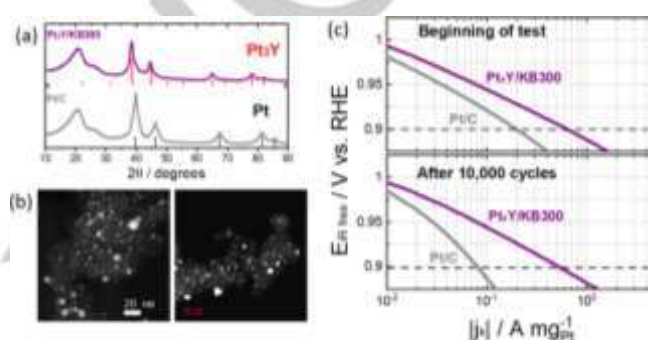
Figure 6 (a) XRD patterns; (b) STEM micrographs; and (c) ORR polarization curves of Pt x Y/KB300. Commercial Pt/C is used as reference in (a) and (c). (Reproduced with permission from ref [40] Copyright 2022, American Chemistry Society).
