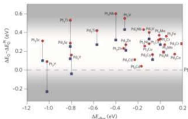
Figure 1. DFT calculated oxygen binding energy (relative to Pt) as a function of the alloying energy. The red circles indicate a 50 % of the alloying metal on the second layer, while the blue squares indicate a 25 % of the alloying metal on the second layer. The grayscale gradient indicates the optimal oxygen adsorption for the ORR process. Reproduced with permission from ref [11] . Copyright 2022, Springer.
