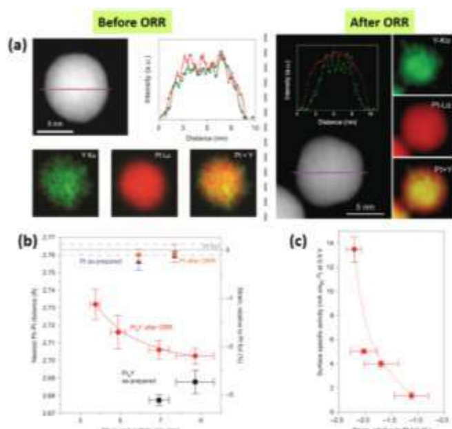
Figure 4 (a) STEM micrographs and elemental analysis (EDS) mapping before and after the AST of 9 nm Pt x Y; (b) average nearest-neighbor Pt-Pt distance as a function of the particle size; and (c) surface specific activity as function of the average compressive strain in the Pt x Y particles relative to bulk Pt. (Reproduced with permission. [26] Copyright 2021, Springer).
