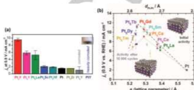
Figure 2 (a) Overall ranking of ORR activity of polycrystalline electrodes of Pt-REM alloys (Reproduced with permission from ref [12] . Copyright 2022, The Royal Society of Chemistry.); and (b) specific activity as function of the bulk lattice parameter (lower axis) and bulk Pt-Pt inter-atomic distance (upper axis). For comparison, it is shown the ORR performance before (darker line) and after (lighter line) the stability test (Reproduced with permission from ref [23] . Copyright 2022).
