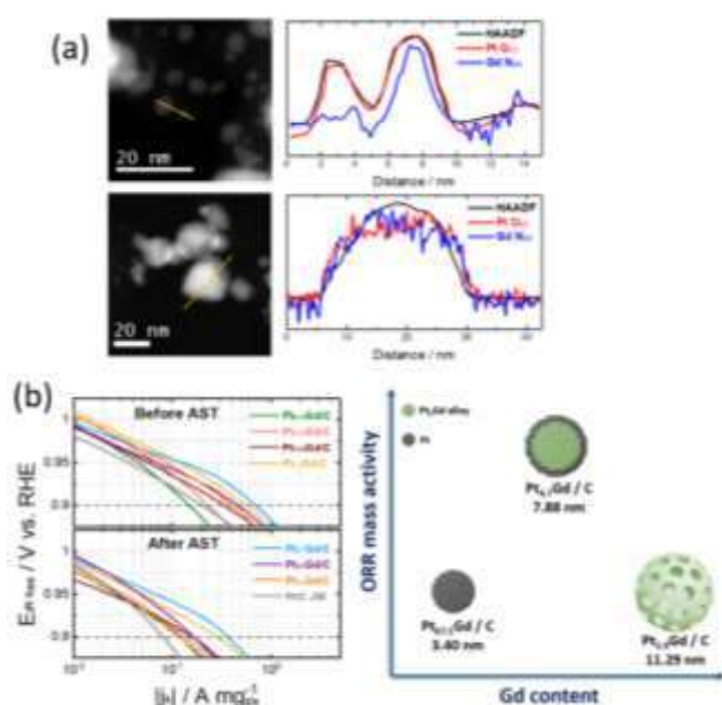
Figure 5 (a) STEM micrographs and the corresponding EELS linear profile of solid NPs and porous nanoarchitectures; and (b) ORR activity ranking of Pt x Gd/C nanostructures. (Reproduced with permission from ref [37] Copyright 2022, American Chemistry Society).
